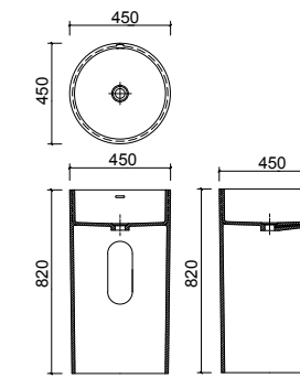
BA050003 450 x 450 x 820mm
