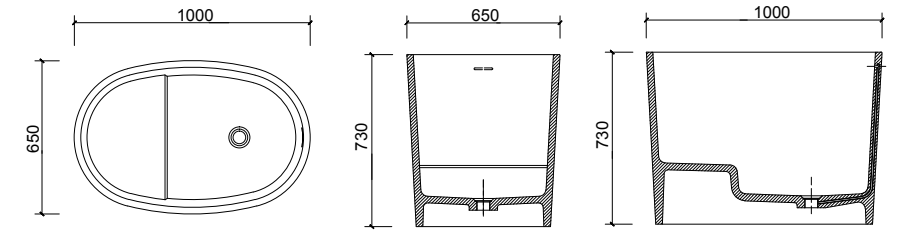
BT030275 1000 x 650 x 730mm
