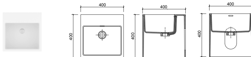
BA040051 400 x 400 x 400mm
