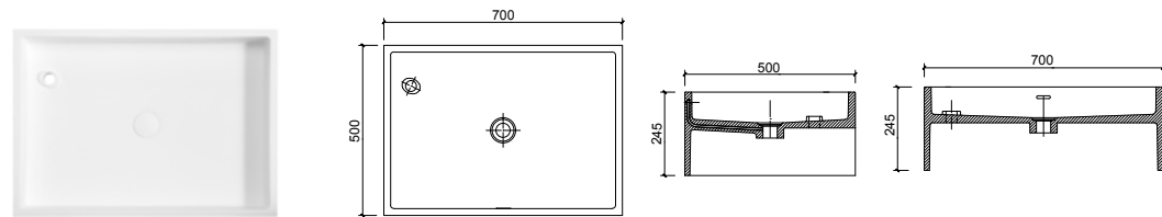
BA020111 700 x 500 x 245mm
