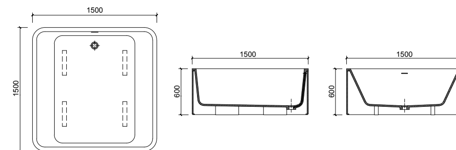
BT020225 1500 x 1500 x 600mm
