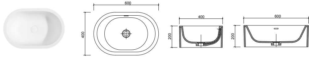
BA030006 600 x 400 x 200mm
