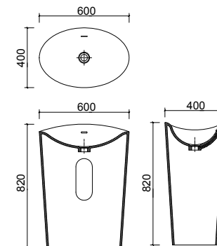
BA050021 600 x 400 x 820mm
