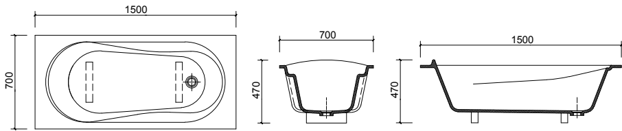
BT020034 1500 x 700 x 470mm
