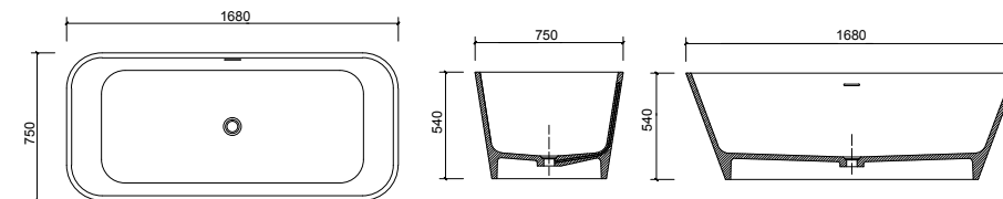
BT020248 1680 x 750 x 540mm
