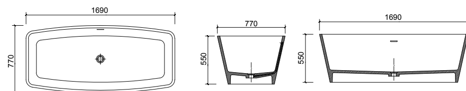
BT040065 1690 x 770 x 550mm
