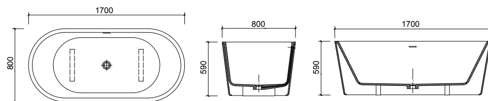
BT030037 1700 x 800 x 590mm
