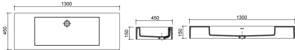
BA060120 1300 x 450 x 150mm
