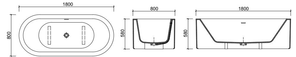
BT030001 1800 x 800 x 580mm
