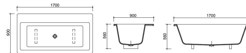
BT020074 1700 x 900 x 560mm
