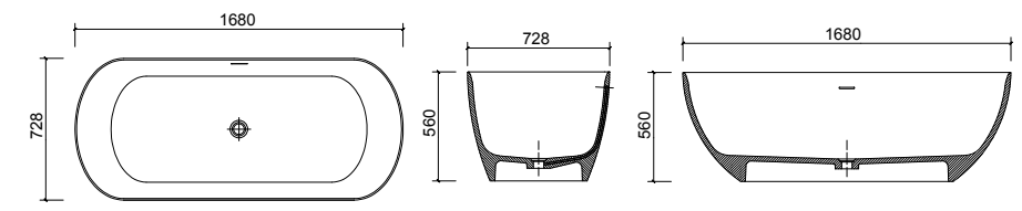
BT030222 1680 x 728 x 560mm
