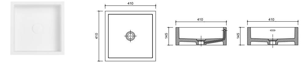
BA020128 410 x 410 x 145mm
