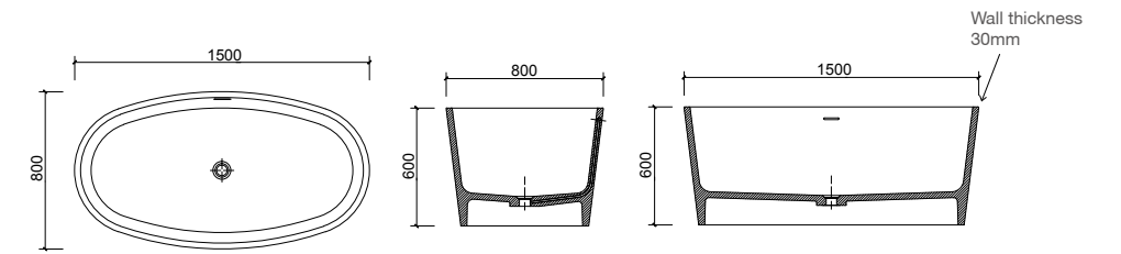
BT030039 1500 x 800 x 600mm
