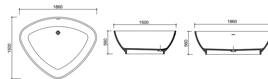
BT040057 1860 x 1500 x 560mm
