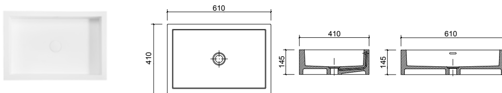
BA020008 610 x 410 x 145mm
