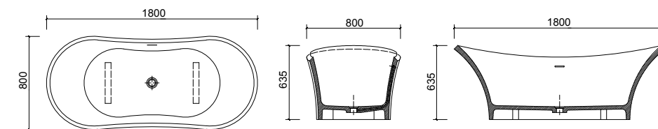
BT040005TH 1800 x 800 x 635mm
