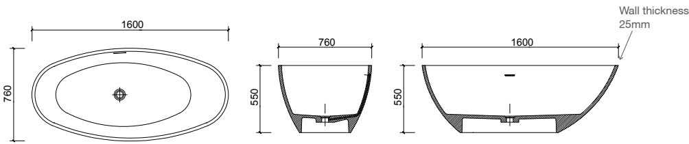
BT030003STH 1600 x 760 x 550mm
