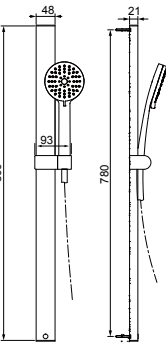
BL7001H Optional sliding bar for hand shower of BL606510H
