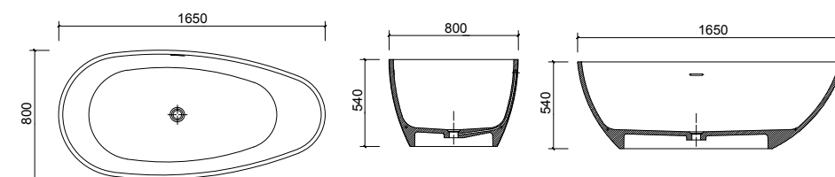
BT040040 1650 x 800 x 540mm
