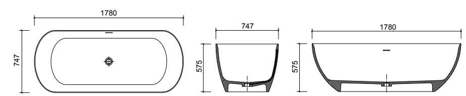
BT030266 1780 x 747 x 575mm
