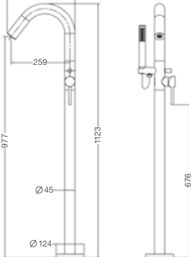
BL316180 Single lever floorstanding bath faucet & shower set
