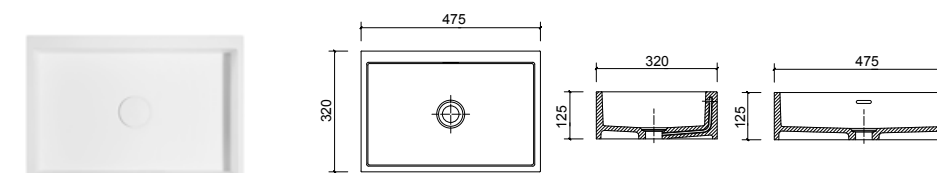
BA020207 475 x 320 x 125mm
