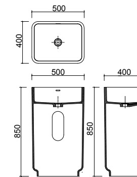
BA050112 500x 400 x 850mm
