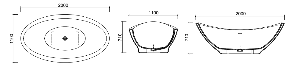
BT030058 2000 x 1100 x 710mm △
