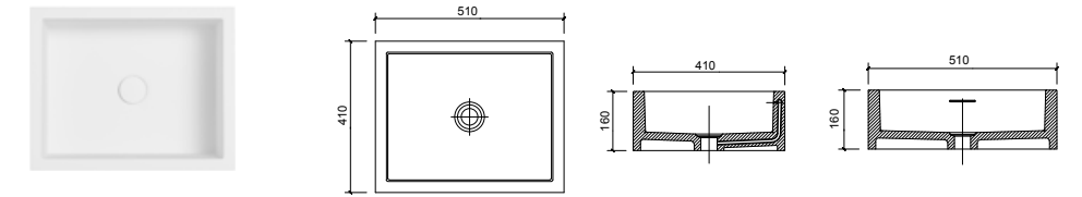
BA020143 510 x 410 x 160mm
