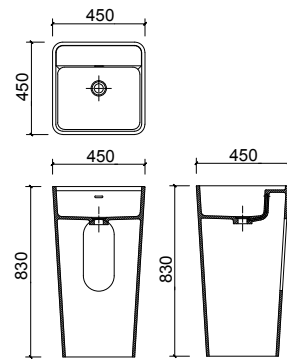
BA050127 450 x 450 x 830mm
