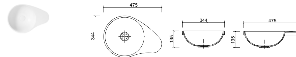
BA040023 475 x 344 x 135mm ★
