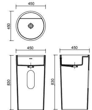
BA050107 450 x 450 x 830mm
