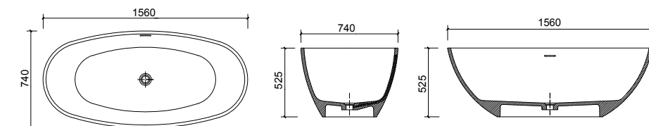
BT030175 1560 x 740 x 525mm
