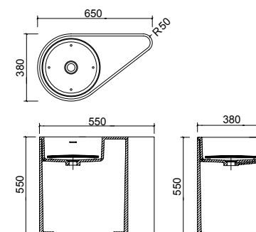
BA040060 with cover 650 x 380 x 550mm
