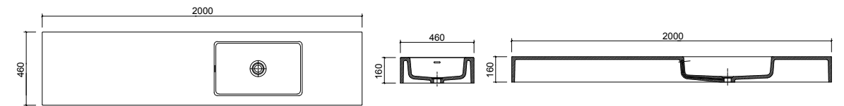
BA060315 2000 x 460 x 160mm
