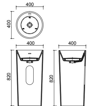
BA050091 with cover 400 x 400 x 820mm
