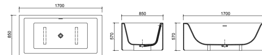
BT020001 1700 x 850 x 570mm
