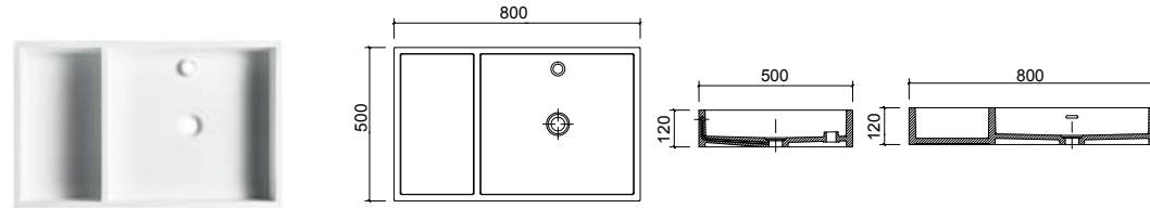
BA060106 800 x 500 x 120mm
