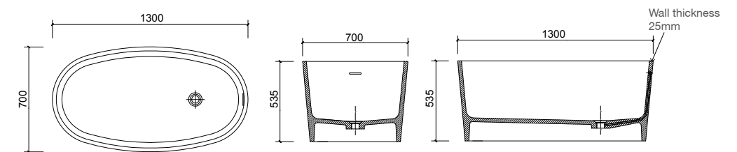
BT030039STH 1300 x 700 x 535mm
