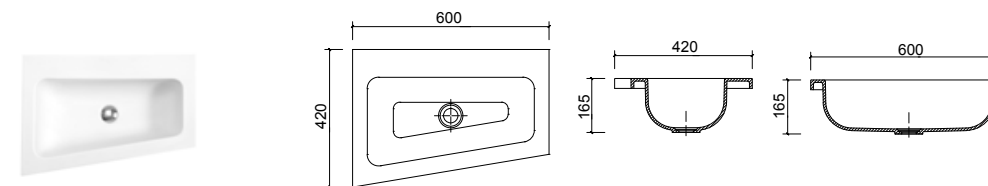
BA040021 600 x 420 x 165mm ★
