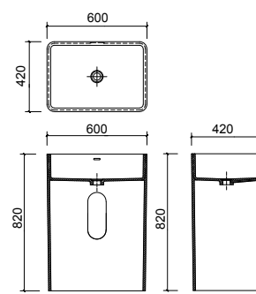
BA050001 600 x 420 x 820mm
