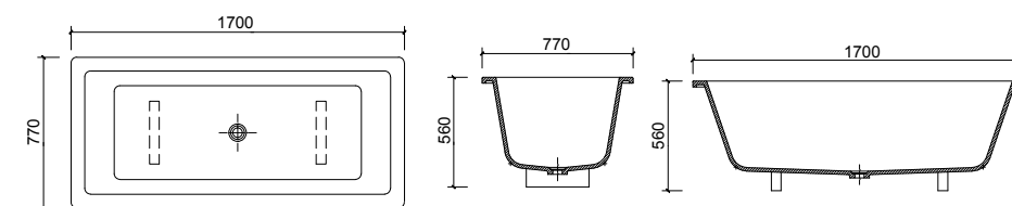
BT020074_R 1700 x 770 x 560mm
