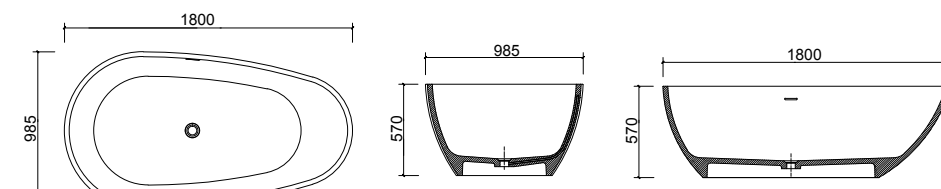
BT040080 1800 x 985 x 570mm
