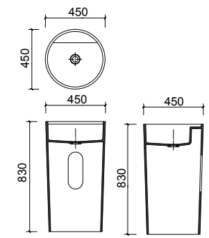
BA050058 450 x 450 x 830mm
