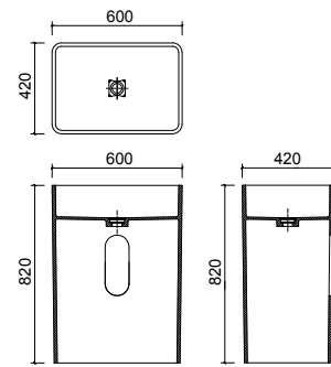
BA050201 600 x 420 x 820mm
