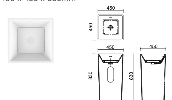
BA050004 with cover 450 x 450 x 830mm
