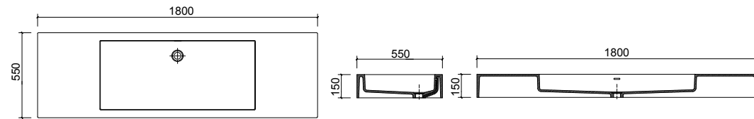
BA060149 1800 x 550 x 150mm
