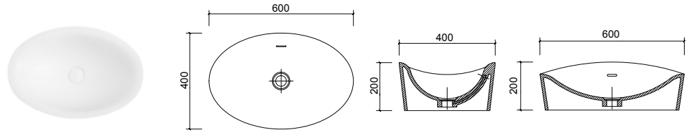
BA030005 600 x 400 x 200mm
