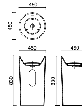
BA050005 with cover 450 x 450 x 830mm
