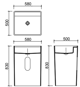
BA050057 580 x 500 x 830mm
