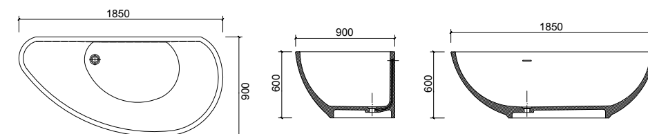
BT040006 1850 x 900 x 600mm
