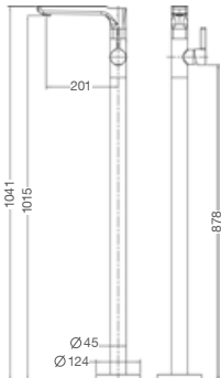
BL323100 Single lever floorstanding bath & lavatory set
